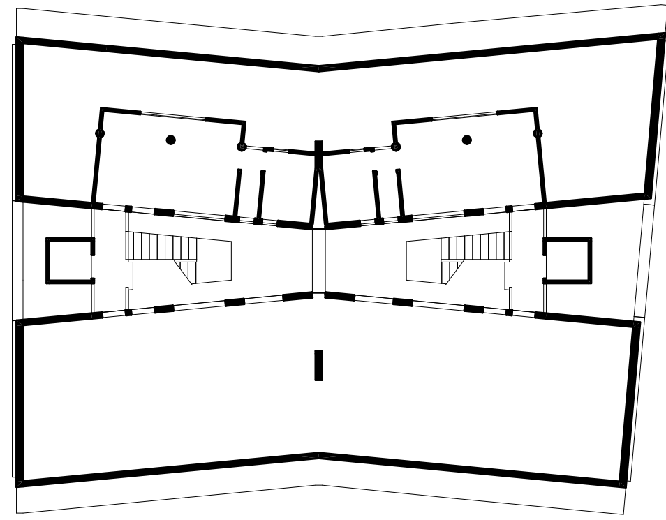
PLAN R+7
