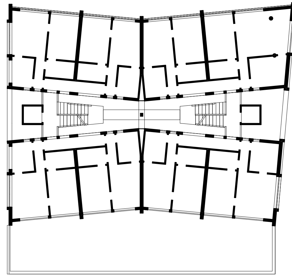
PLAN R+4
