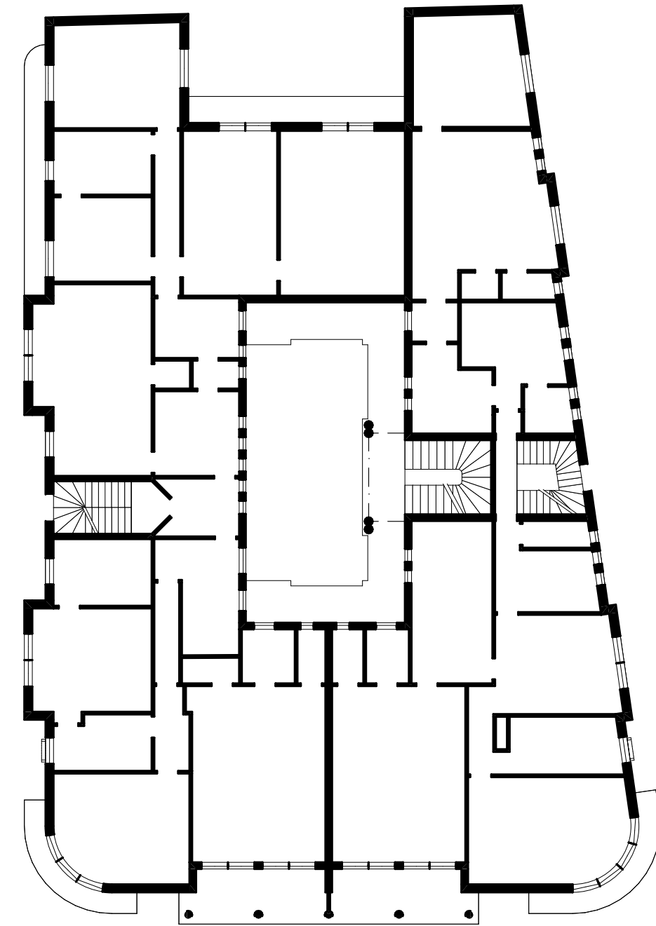
PLAN R+3
