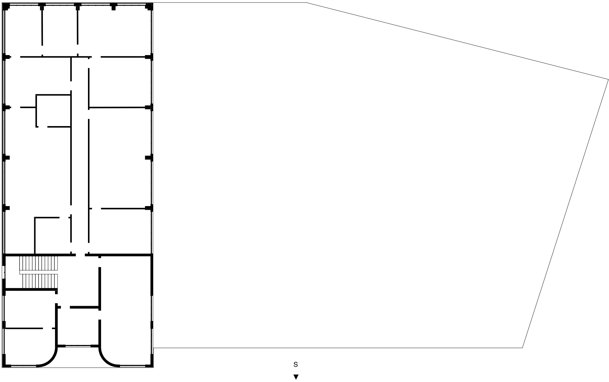
PLAN R+1
